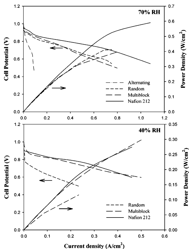
Figure 6. Hydrogen–air fuel cell performance of the alternating, random, and multiblock PEMs at 100 °C with gas inlet humidification at 70% (top) and 40% (bottom) (Nafion is shown for comparison).
